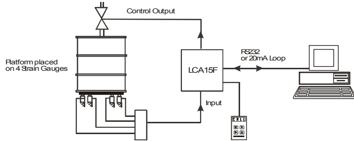
Figure 1.2 Drum Filling
