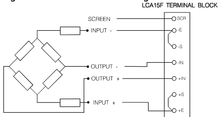
Figure 2.2 The 4 Wire Strain Gauge
