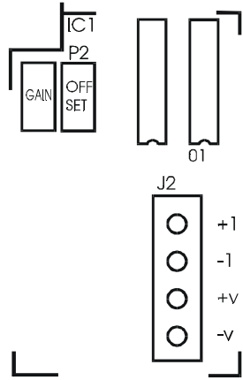
Figure 5.3 - UAFAO Connections
