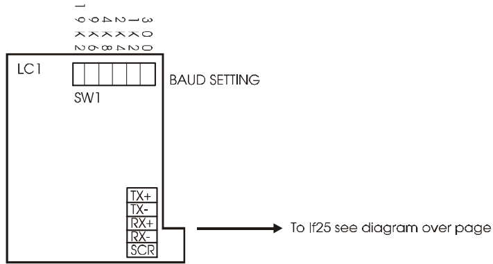
Figure 7.1 LC1 Current Loop
