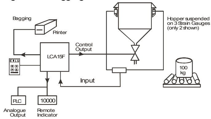
Figure 1.1 Bagging
