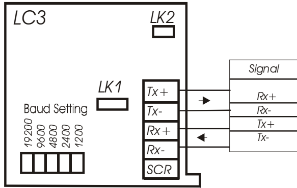
Figure 7.3 The LC3 Isolated RS232/485 - RS485 Mode Connections
