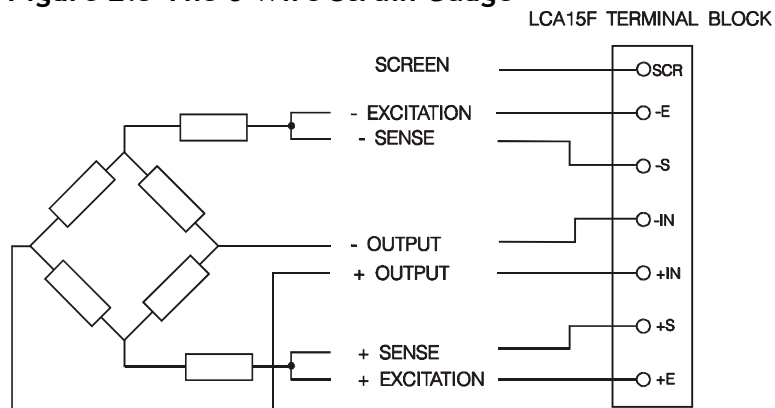
Figure 2.3 The 6 Wire Strain Gauge
