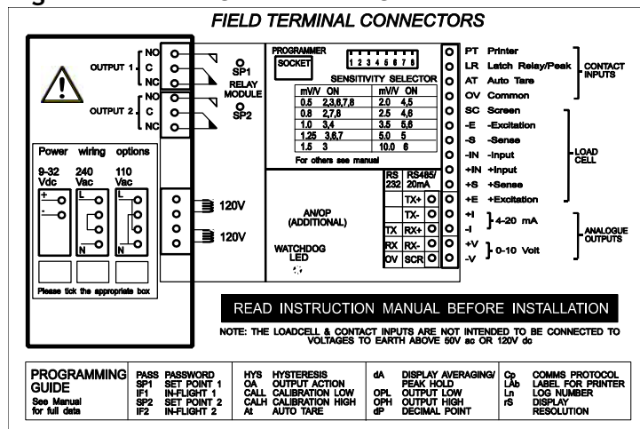
Figure 2.1 The LCA15F Field Connection Terminals
