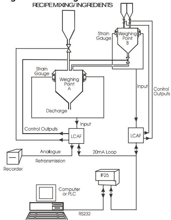
Figure 1.3 Mixing Control
